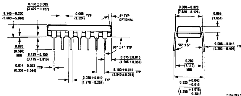
14-Lead Molded Dual-In-Line Package (N) Order Number DM74LS54N NS Package Number N14A
