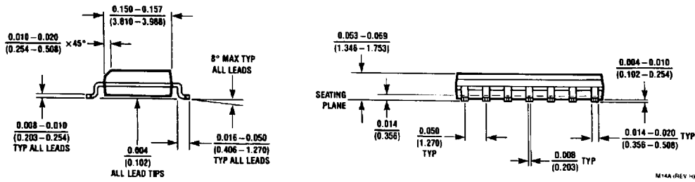
14-Lead Small Outline Molded Package (M) Order Number DM74LS54M NS Package Number M14A
