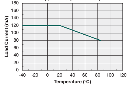
Maximum Load Current vs. Temperature ( I_F=0\text{mA} , I_L=AC\text{ Peak} )
