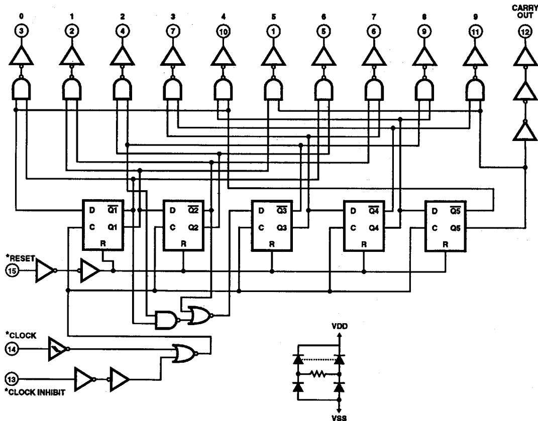
FIGURE 1. CD4017BMS
