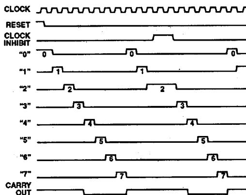
FIGURE 4. CD4022BMS
