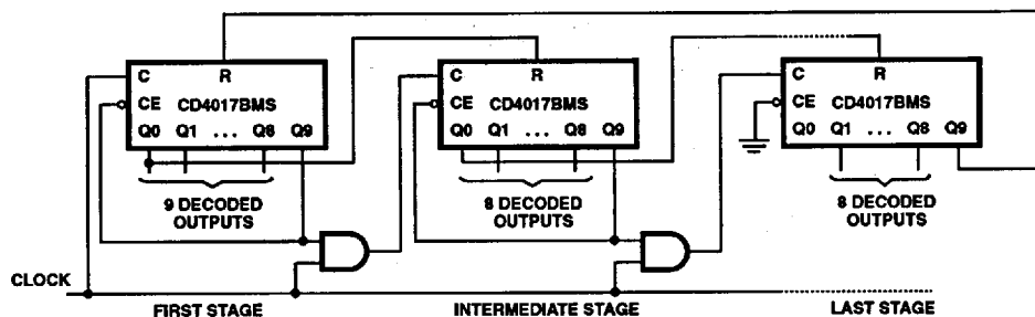
FIGURE 15. CASCADING THE CD4017BMS
