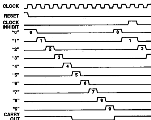
FIGURE 3. CD4017BMS
