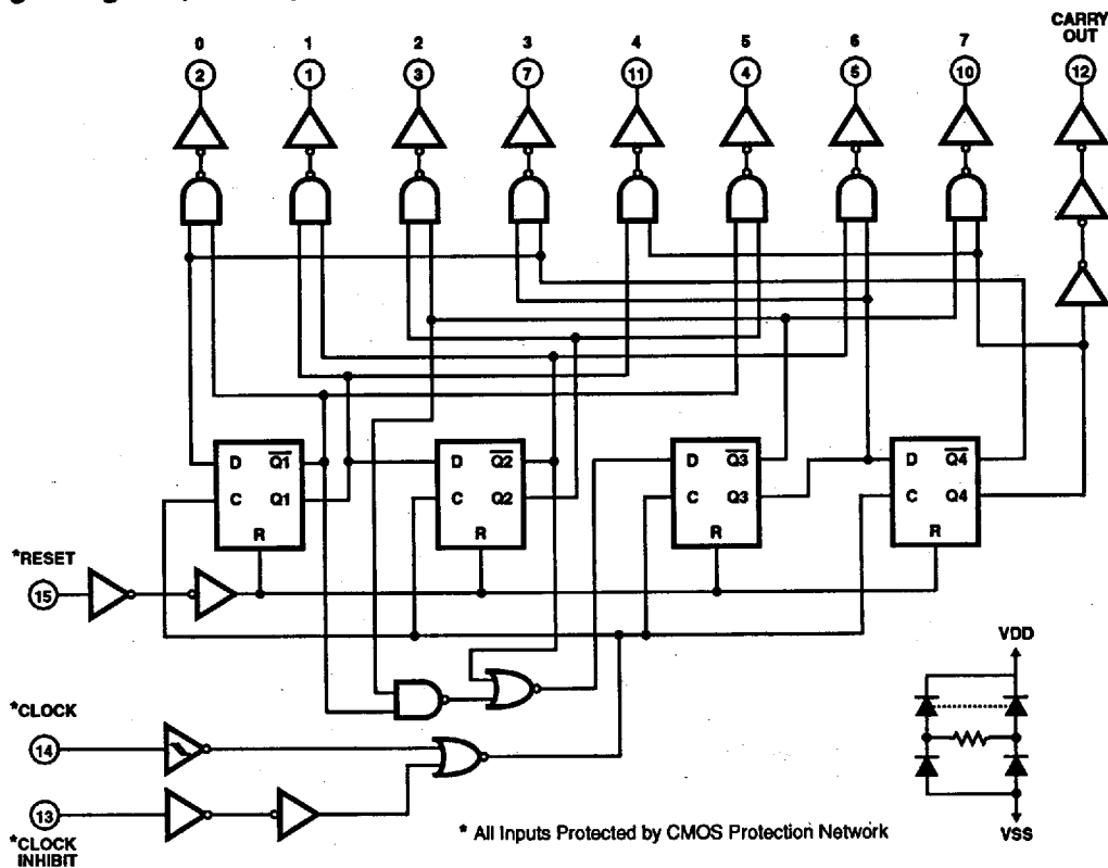
FIGURE 2. CD4022BMS
