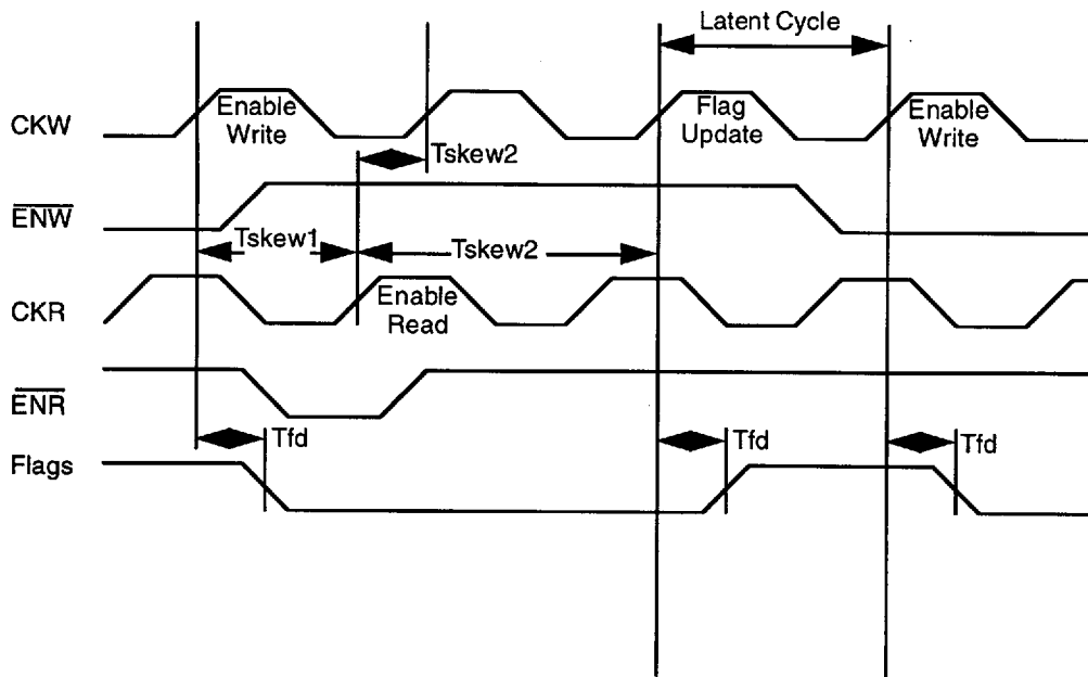
Figure 5. Write Flag Update Timing
