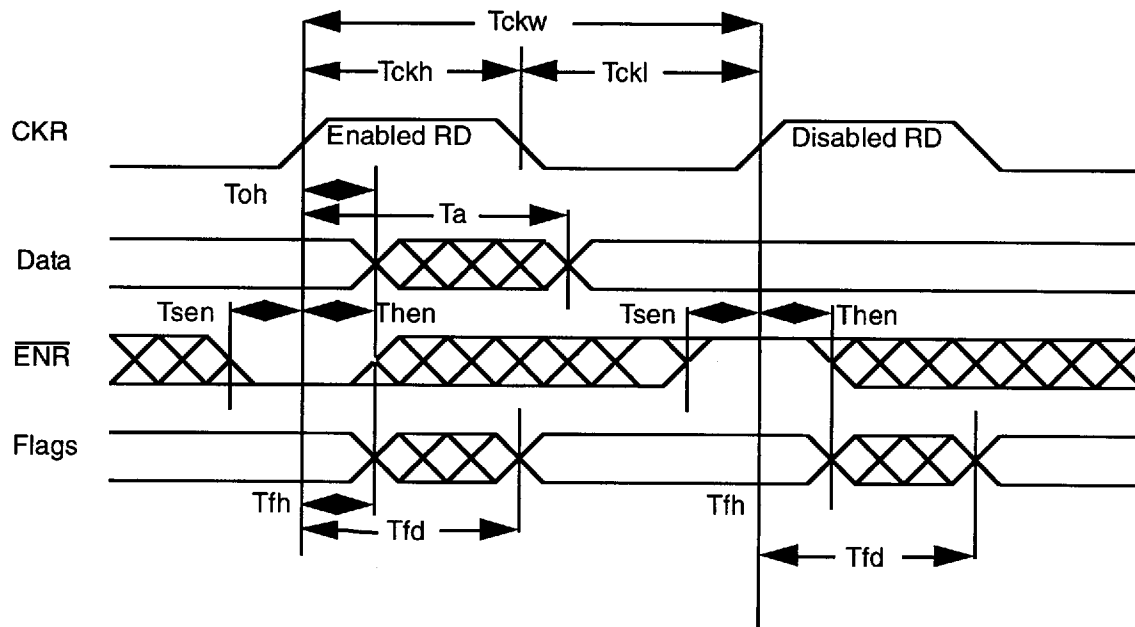
Figure 2. Read Timing
