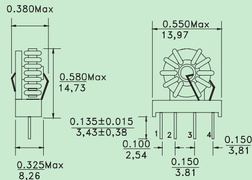
TRANSFORMER
