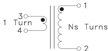
TRANSFORMER
