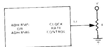
FIGURE 5. OPTIONAL CLOCK RATE FINE ADJUSTMENT
