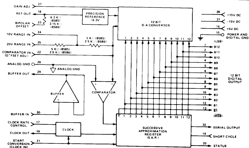
FIGURE 1. ADH-8585 AND ADH-8586 BLOCK DIAGRAM
