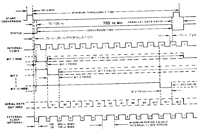
FIGURE 4. ADH-8585 AND ADH-8586 TIMING DIAGRAM
