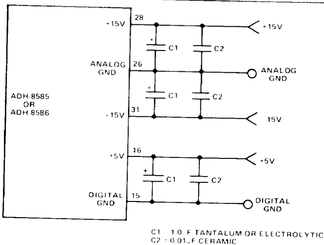
FIGURE 7. POWER SUPPLY DECOUPLING CAPACITORS
