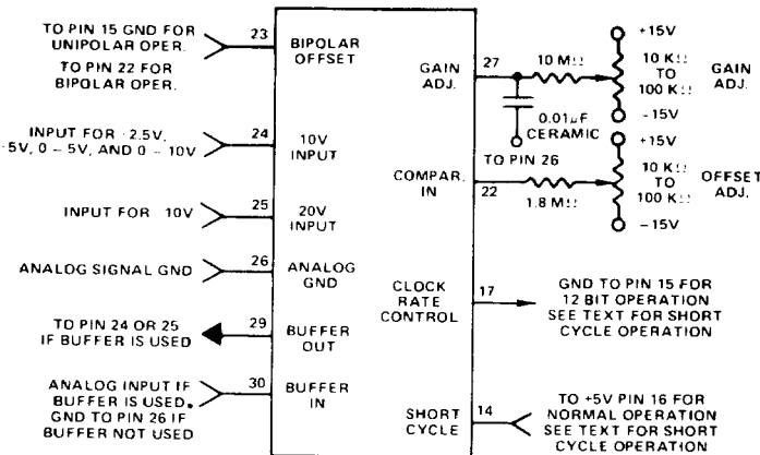
FIGURE 2. CONNECTIONS FOR NORMAL OPERATION
