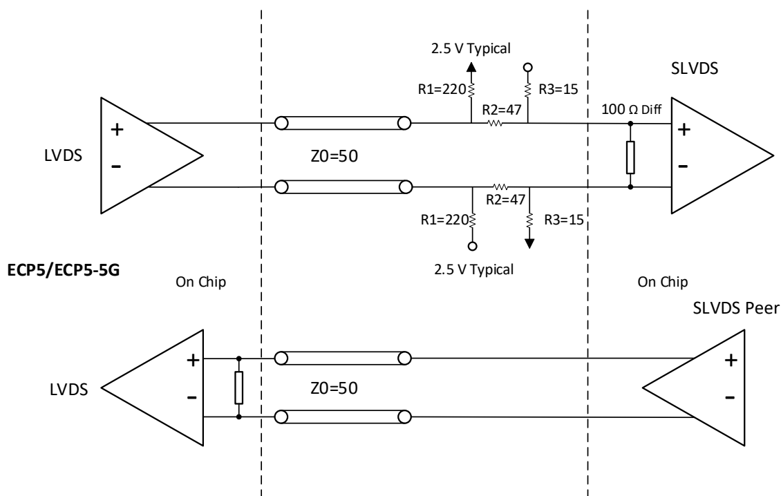
Figure 3.5. SLVS Interface
