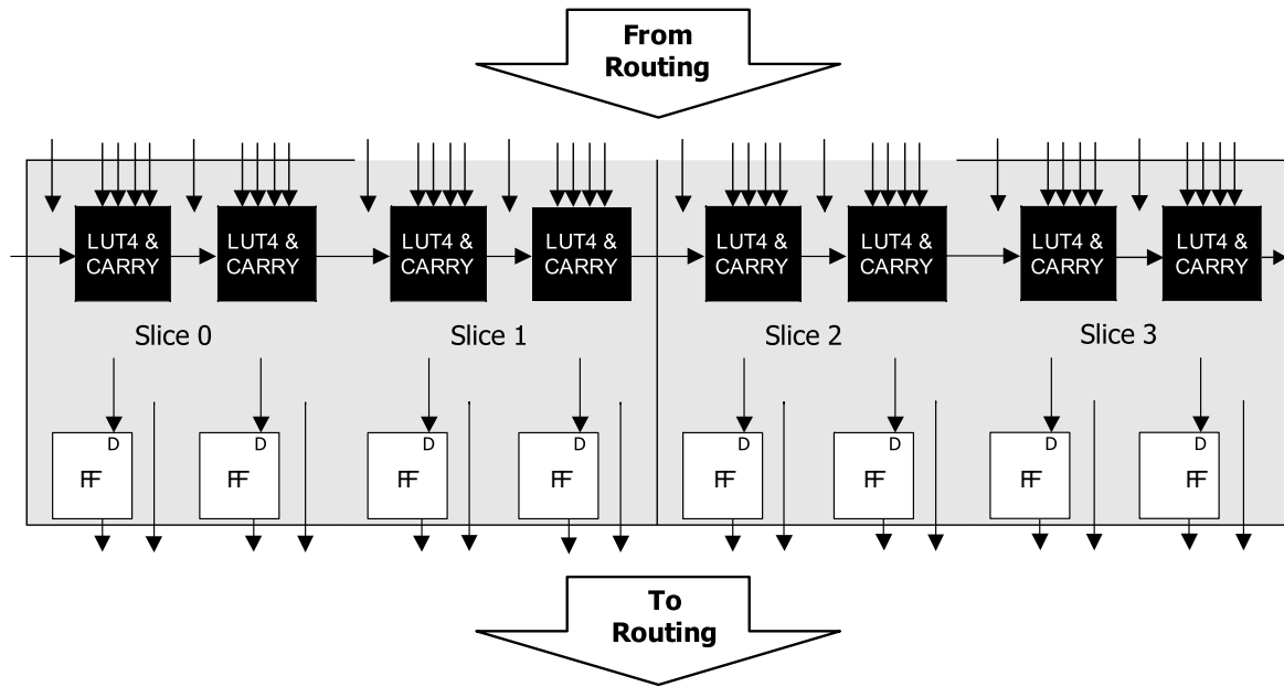
Figure 2.2. PFU Diagram
