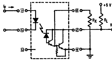
Circuit Diagram - External Base Resistor - R_X
