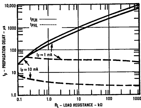
Propagation Delay vs Load Resistance
