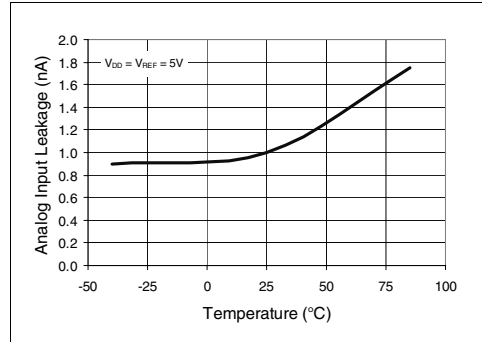
FIGURE 2-39: Analog Input Leakage Current vs. Temperature.
