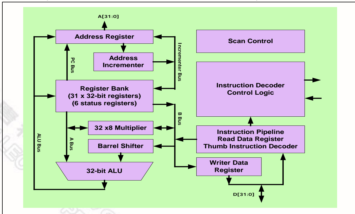
Figure 6.1.1 ARM7TDMI CPU Core Block Diagram
