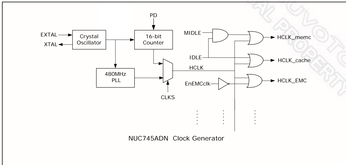
Figure 6.2.6 NUC745 system clock generation diagram
