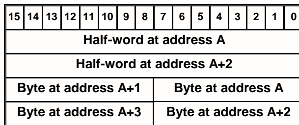
Figure 6.2.2 Little endian addresses of bytes and half-words within half words
