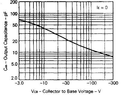
OUTPUT CAPACITANCE vs. COLLECTOR TO BASE VOLTAGE
