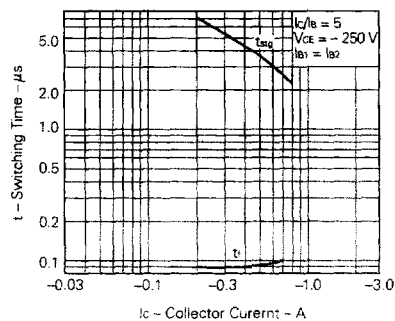
TURN OFF TIME vs. COLLECTOR CURRENT
