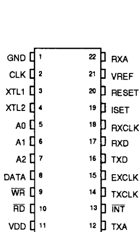
400-Mil 22-Pin DIP
