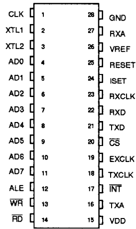
600-Mil 28-Pin DIP
