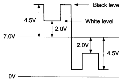
Vsig waveform
