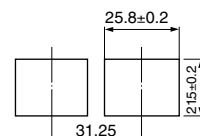
Panel cutting
