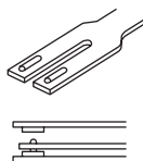
Bifurcated contact
