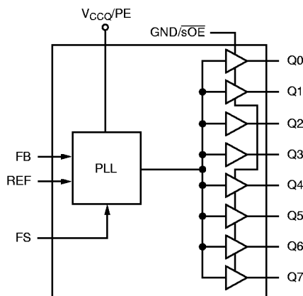
Figure 1. QS59910, QS59920: Logic Block Diagram
