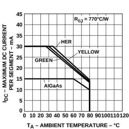
Figure 4. Maximum allowable DC current vs. ambient temperature.
