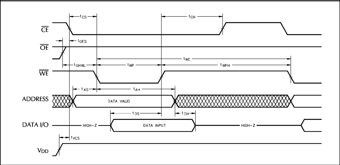
Figure 6: WRITE CYCLE
