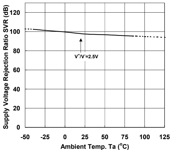
Supply Voltage Rejection Ratio vs. Ambient Temp.
