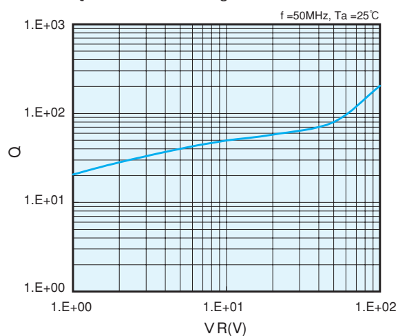
Q vs. Reverse Voltage
