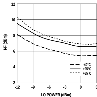
Figure 33. NF vs. LO Power.
