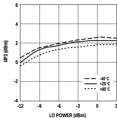
Figure 32. IIP3 vs. LO Power.
