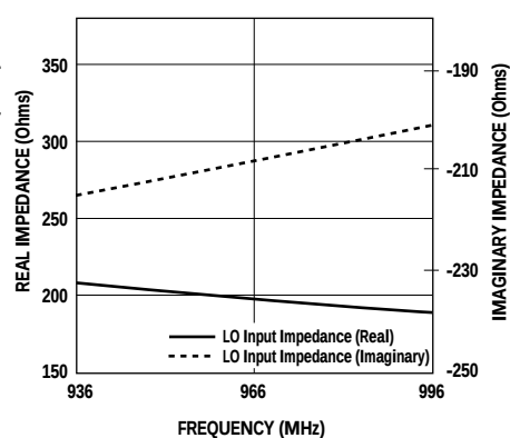
Figure 29. LO Input Impedance (differential) vs. Frequency. [1]
