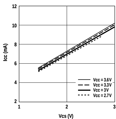
Figure 37A. Icc vs. Vcs.
