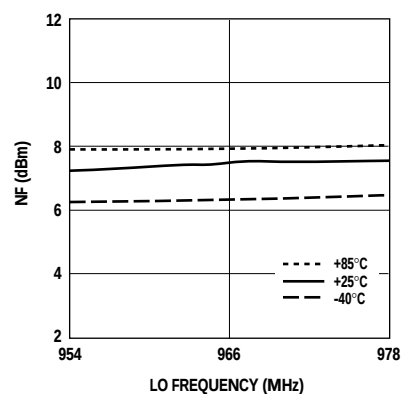
Figure 36. NF vs. LO Frequency.
