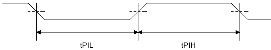
Figure 5 Pulse input timing wave.
