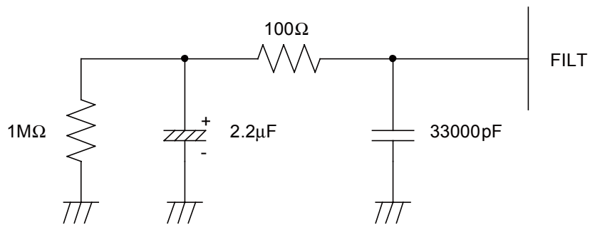
Figure 6 FILT recommended circuit.
