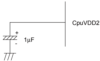
Figure 7 CpuVDD2 recommended circuit.
