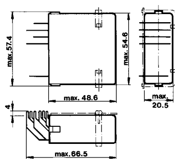
4 POLE PACKAGE
