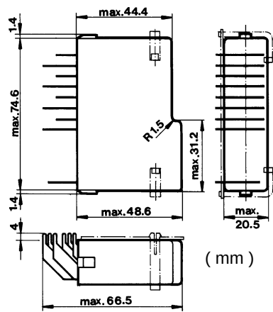
8 POLE PACKAGE
