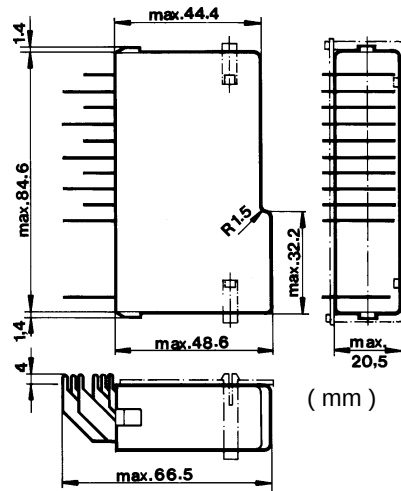
10 POLE PACKAGE
