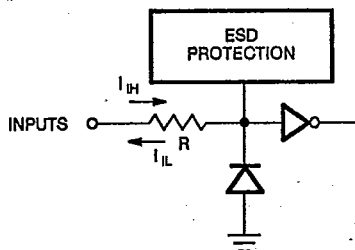
Figure 11. Input Structure (All Inputs)
