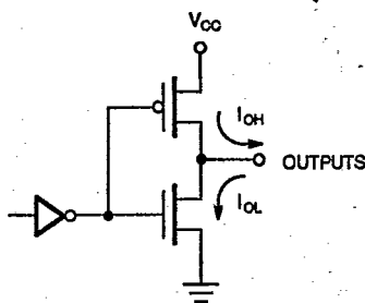
Figure 12. Output Structure
