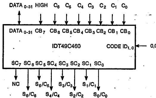
Figure 1. 32-Bit Configuration
