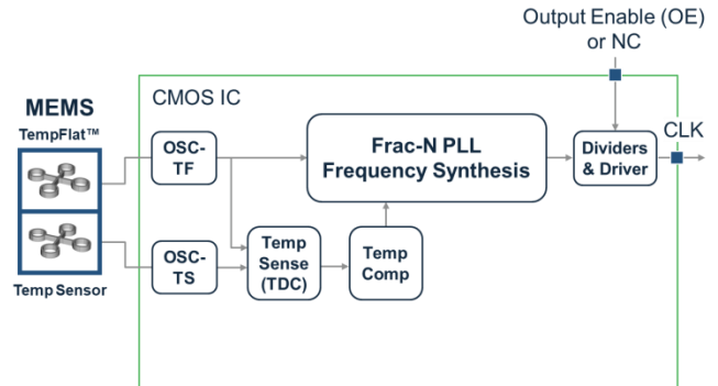
Figure 21. Block Diagram – TCXO
