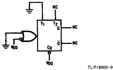
FIGURE 5. Connection of Unused Sections
