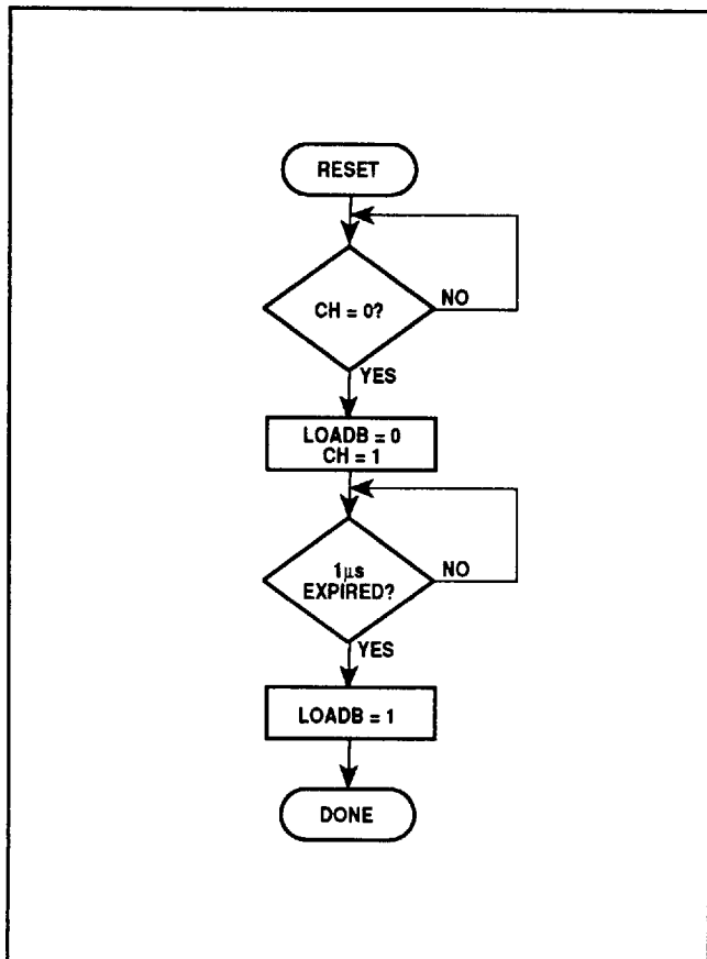
Fig. 10 Channel selection
