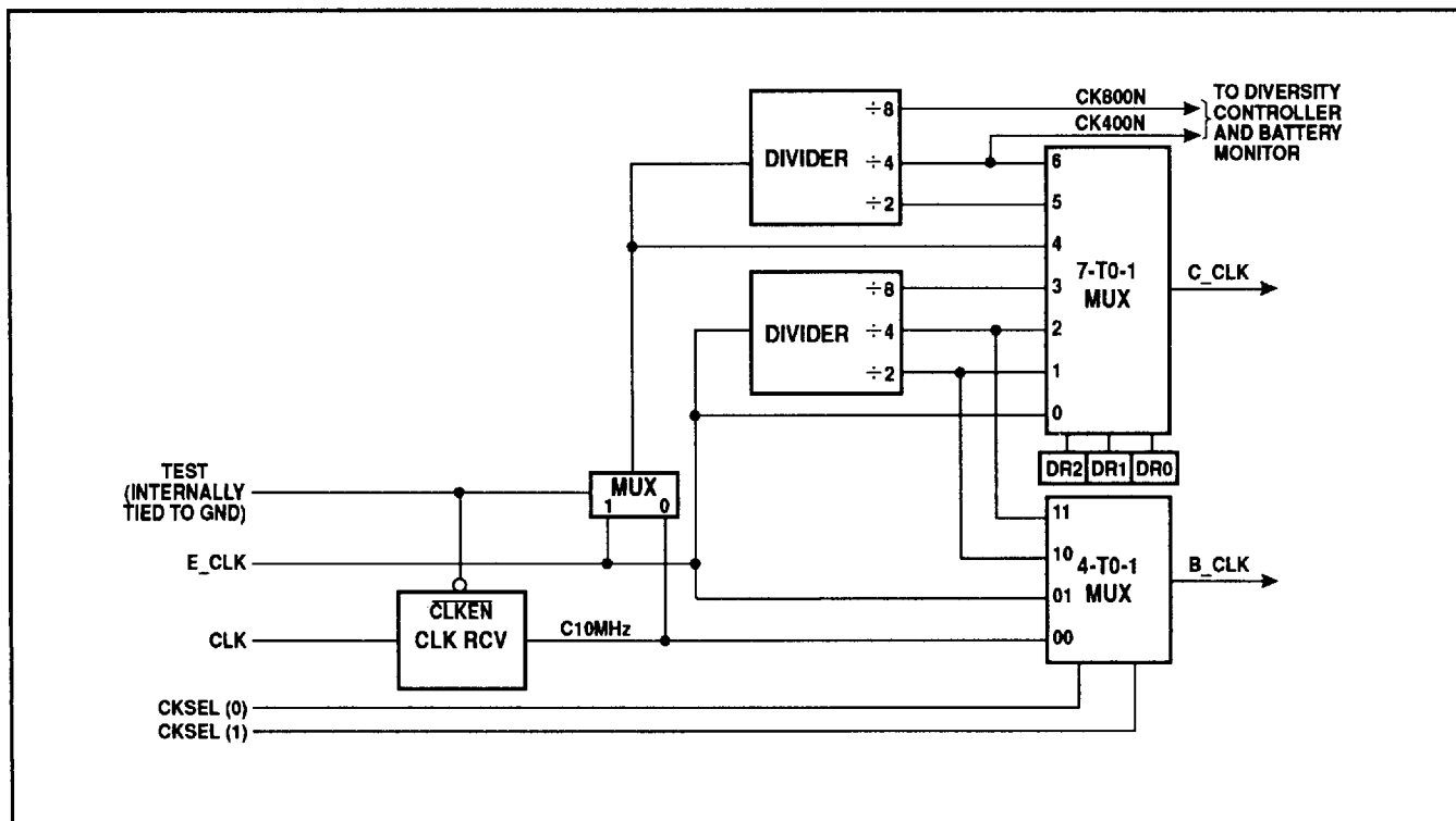
Fig. 14 Clock selector/generator
