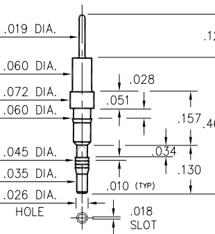
5604-0-01-XX-00-00-03-0 Compliant press-fit in .040±.003 plated hole. For .060→.100 thick board.
