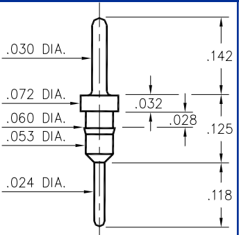
5016-0-00-XX-00-00-03-0 Press-fit in .057 mounting hole
