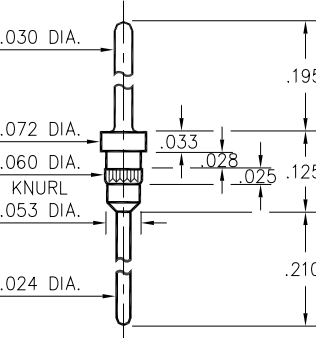
5005-0-00-XX-00-00-03-0 Press-fit in .057 mounting hole
