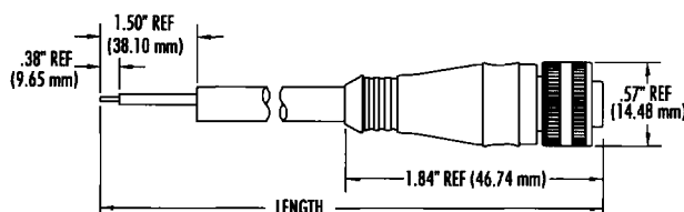
Straight Male Plug / 5 Pole
