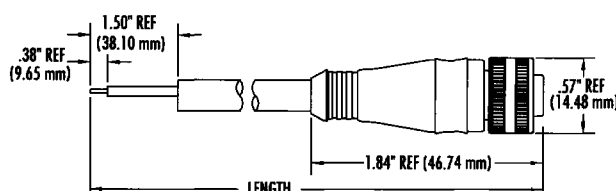
Straight Female Plug / 5 Pole
