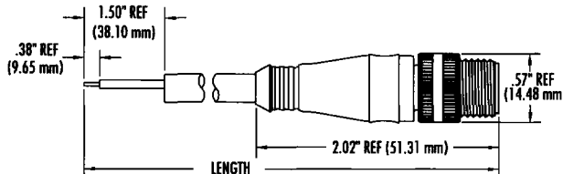
Male Plug with External Threads / 5 Pole
