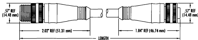
Male/Female Cable Assemblies
