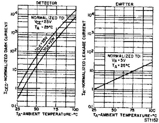
Fig. 4. Leakage Current vs. Temperature
