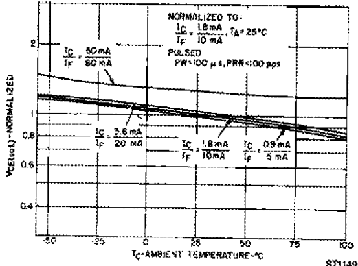
Fig. 3. V_{CE(sat)} vs. Temperature
