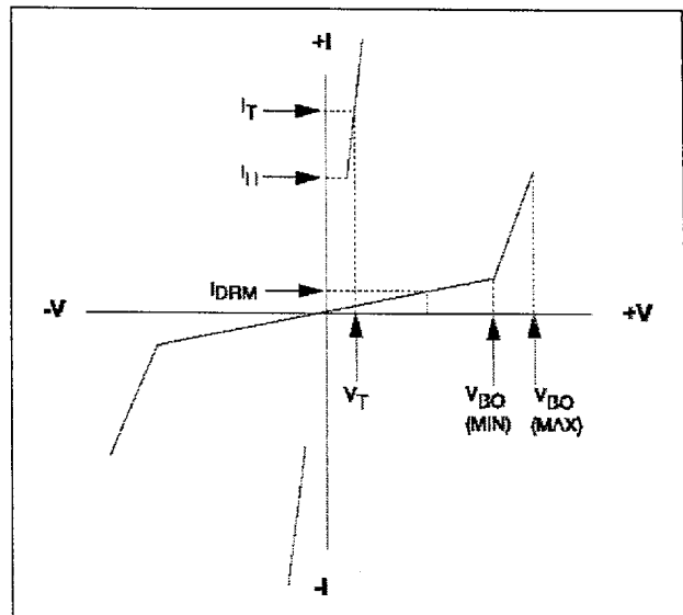
V-I Characteristics
