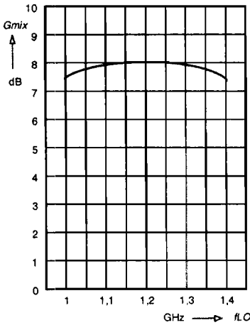
Conversion Gain Gmix = f(fLO)
