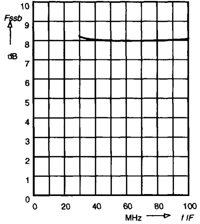
SSB Noise Figure F_{ssb} = f(f\ I/F) fLO = 1185MHz; PLO = -2dBm; fRF = fLO+fIF
