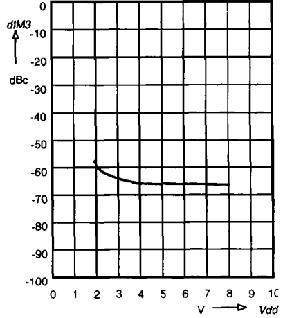
Third Order IMD dIM3 = f(Vdd)
