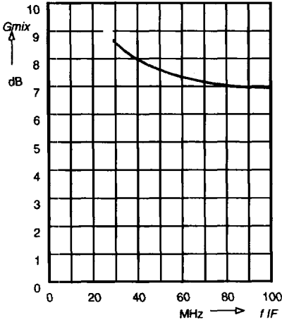
Conversion Gain G_{mix} = f(f\ I/F) fLO = 1185MHz; PLO = -2dBm; fRF = fLO+fIF
