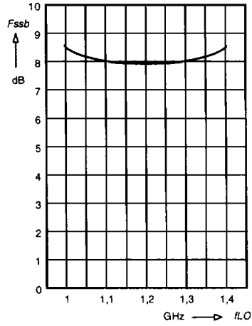
SSB Noise Figure Fssb = f(fLO)
