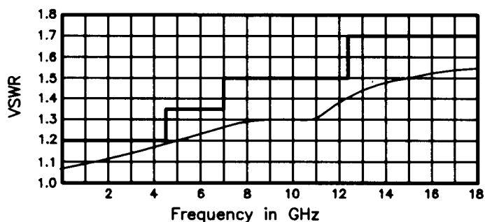
VSWSR Vs. Frequency
