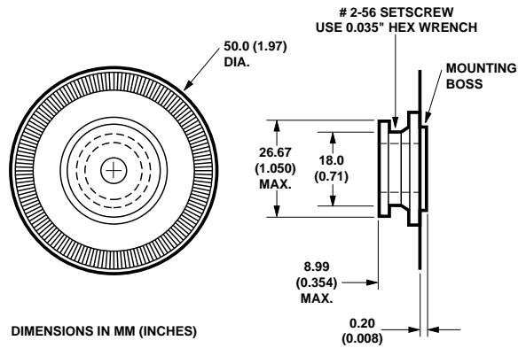
Figure 5. HEDS-6100 Codewheel.
