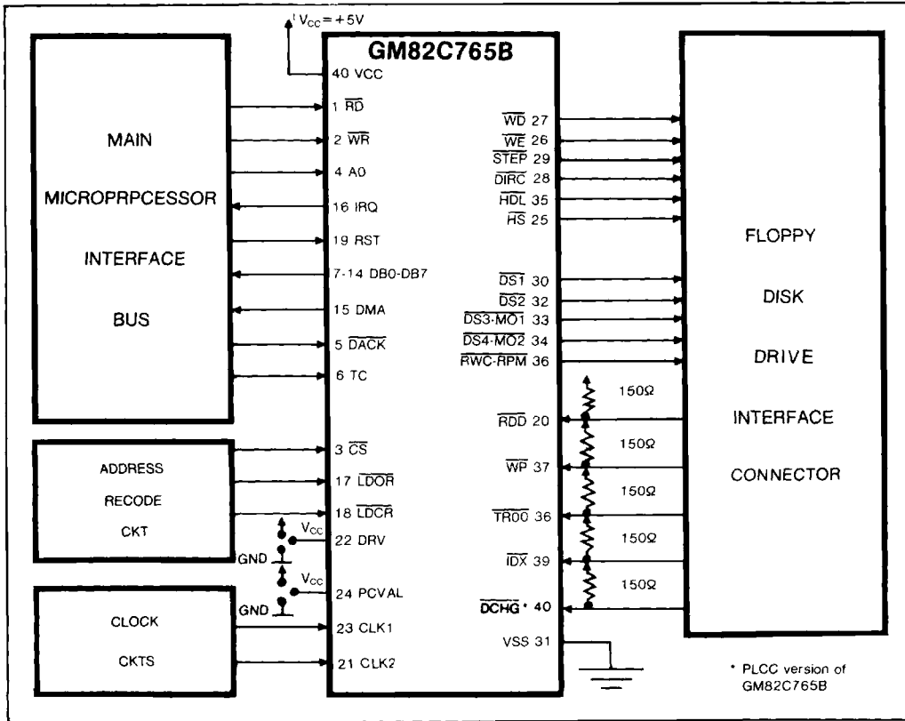
Fig. 2. TYPICAL GM 82C765B APPLICATION SYSTEM.
