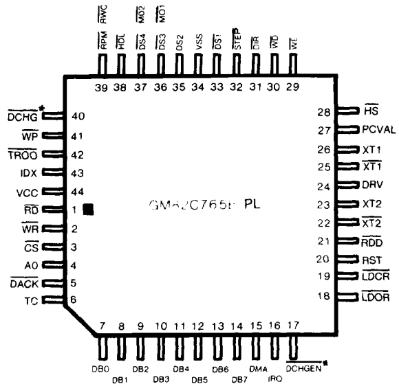
44 PIN PLCC
