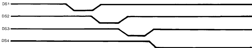
Fig. 4. Drive select polling timing
