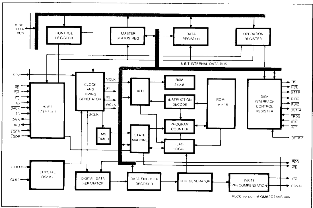
Fig 1. GM82C765B Internal Block Diagram
