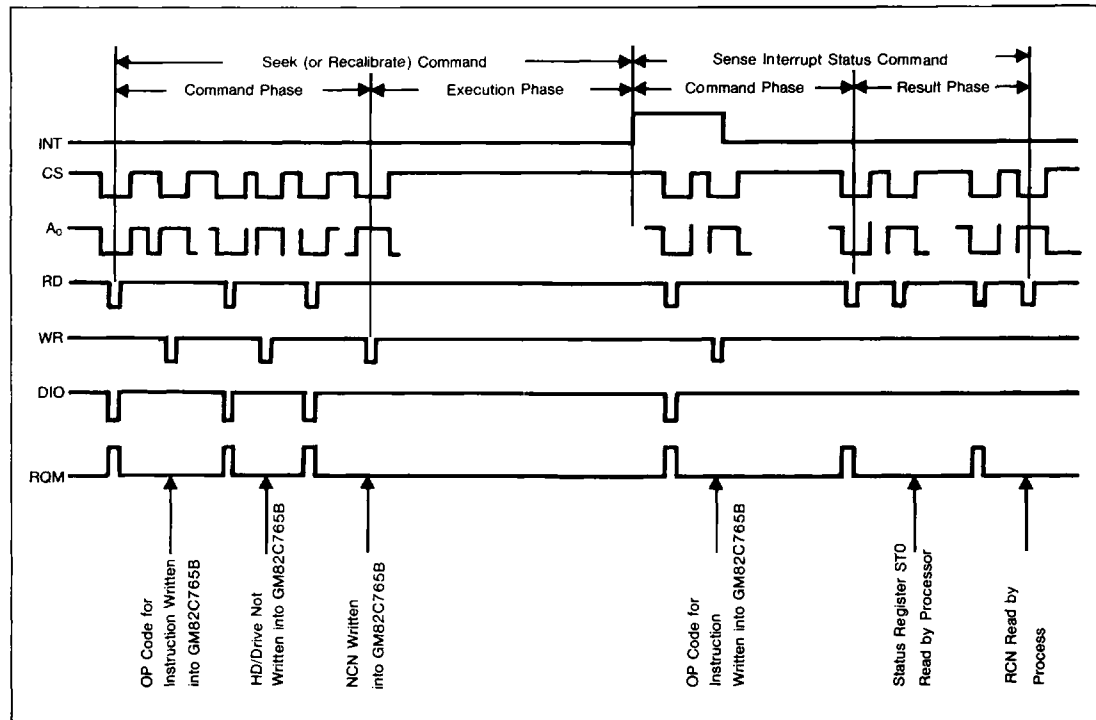
Fig. 7. Seek, Recalibrate and Sense Interrupt Relationship
