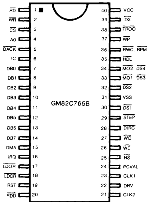
40 PIN DIP
