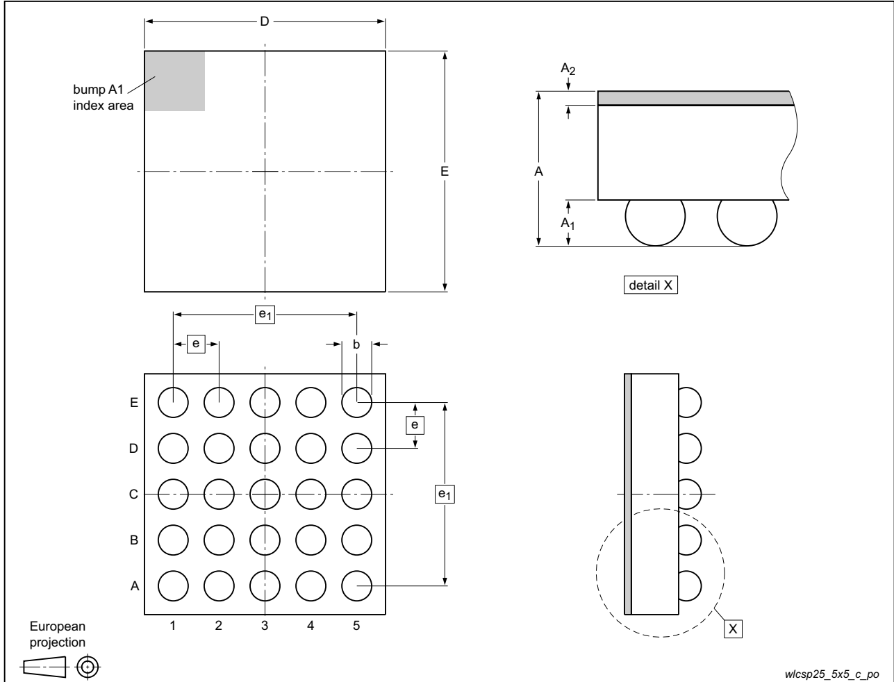
Fig 10. Package outline IP4856CX25/C (WLCSP25 with back side coating)
