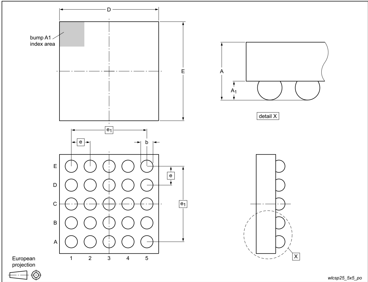
Fig 9. Package outline IP4856CX25 (WLCSP25)
