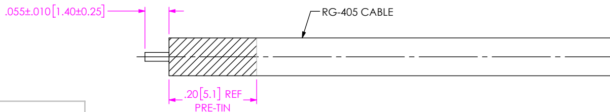
IN-PROCESS VIEW 1
