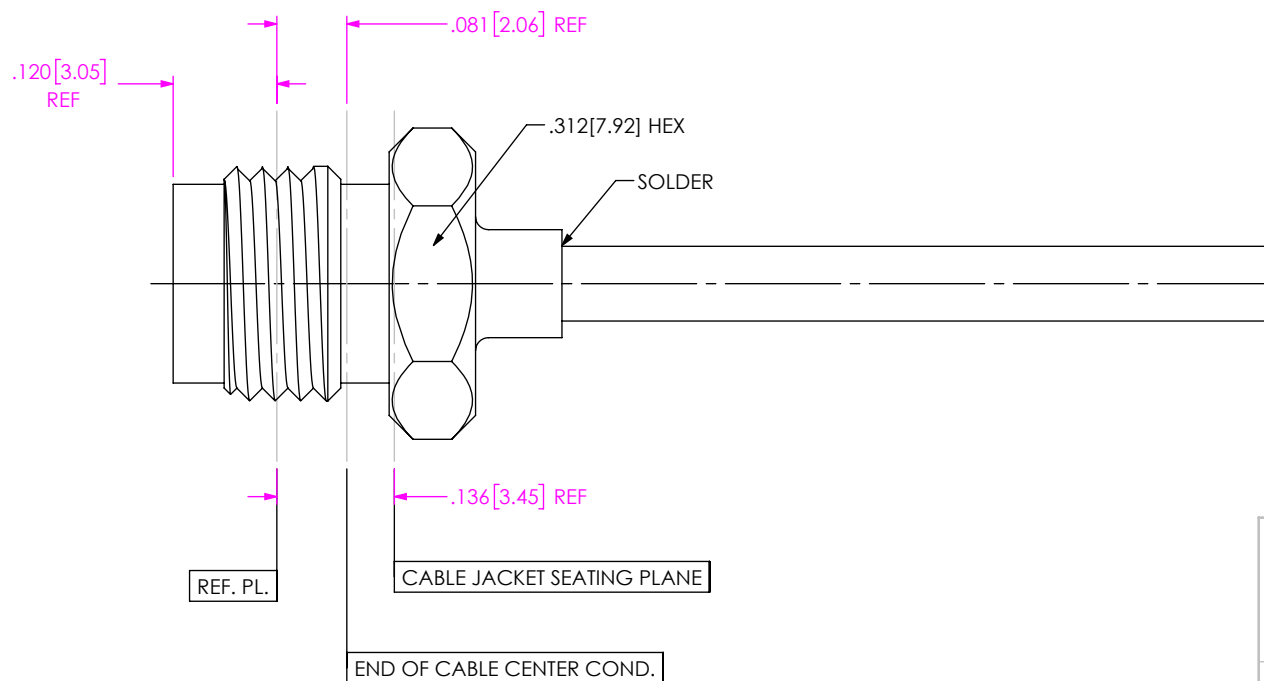
IN-PROCESS VIEW 3
