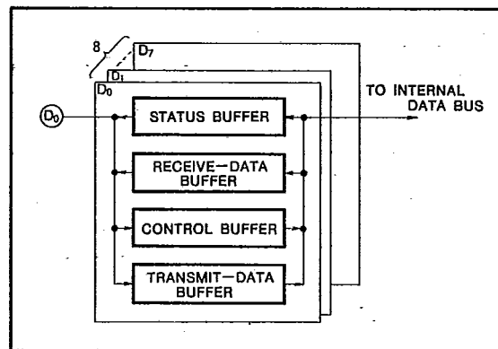
Fig. 2 Data-bus-buffer structure
