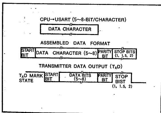
Fig. 6 Asynchronous transmission format I (transmission)
