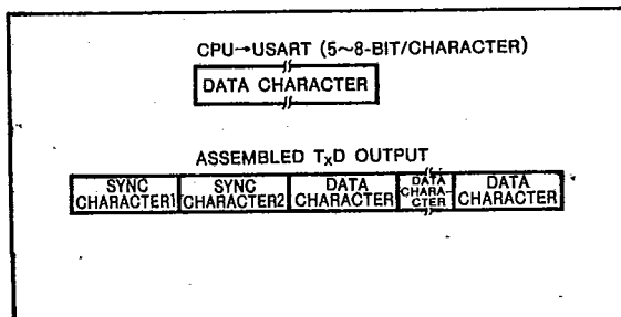
Fig. 8 Synchronous transmission format I (transmission)
