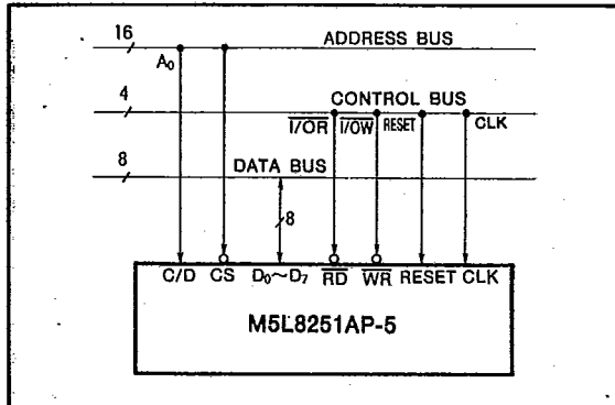
Fig. 1 M5L8251AP-5 Interface to CPU system bus
