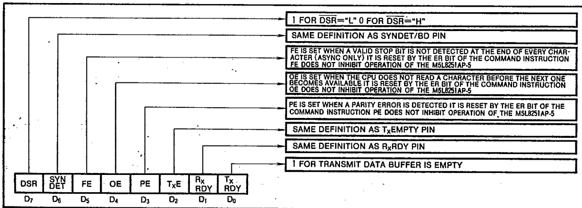
Fig. 10 Status information (C/D="H", WR="L")
