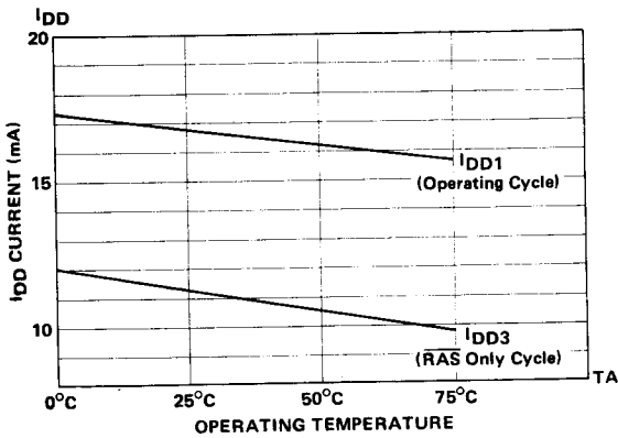
TYPICAL I_{DD} CURRENT VS. OPERATING TEMPERATURE
