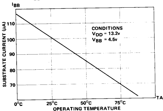
TYPICAL I_{BB} CURRENT VS. OPERATING TEMPERATURE
