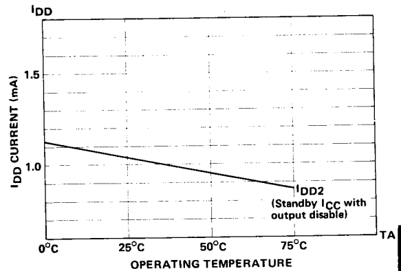
TYPICAL I_{DD} CURRENT VS. OPERATING TEMPERATURE
