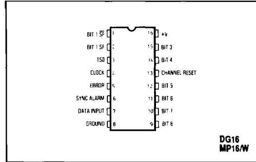
Fig.1 Pin connections
