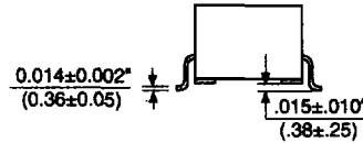
END VIEWS
