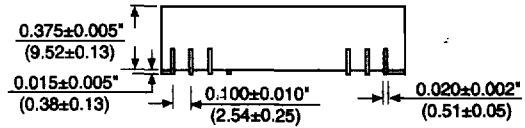
SIDE VIEWS
