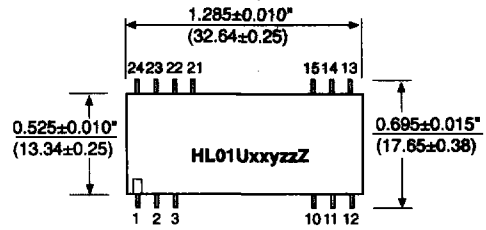
TOP VIEWS
