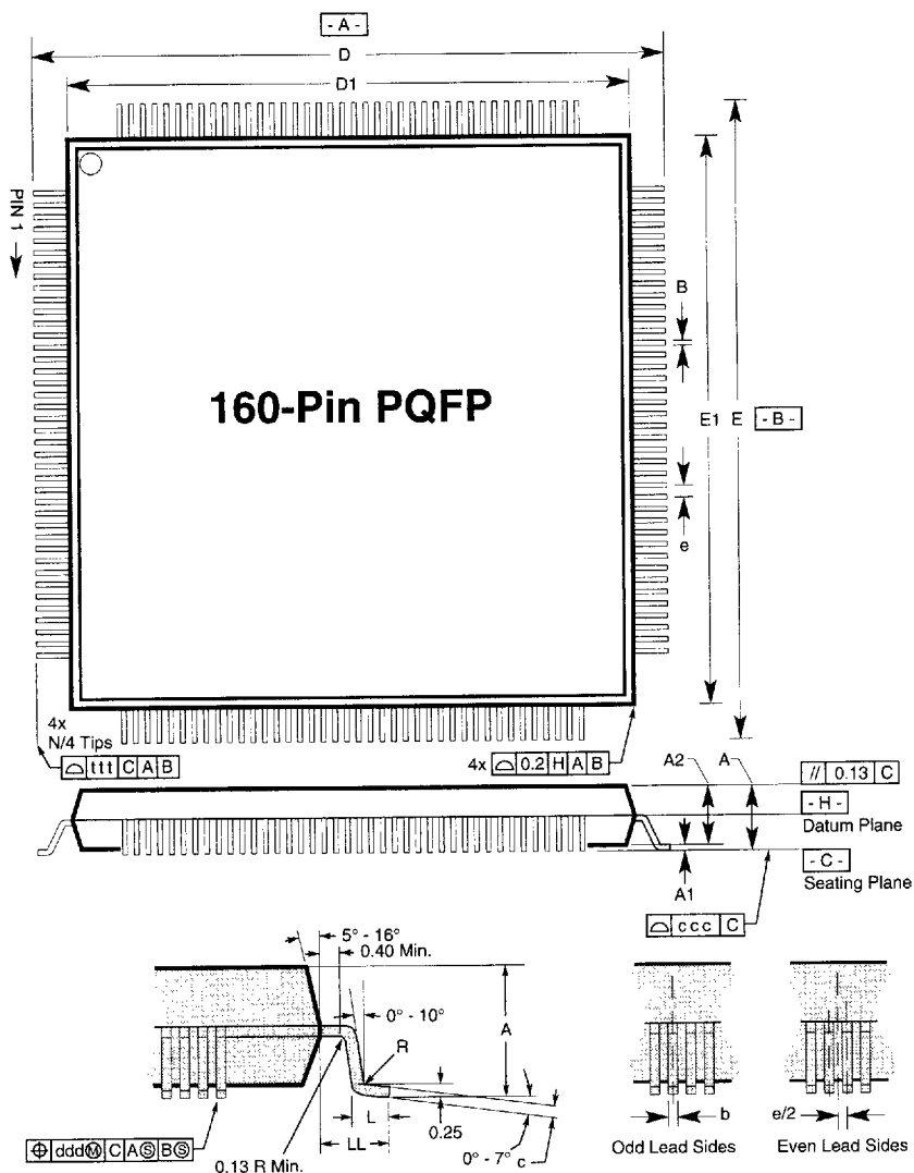
Figure 7-1 Package Dimensions
