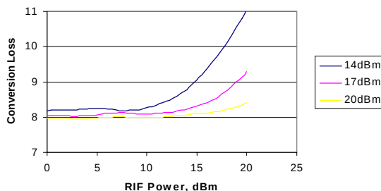
Conversion Loss Compression Curves RF=1.95GHz, LO=1.75GHz, Up-conversion
