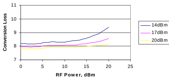
Conversion Loss Compression Curves RF=1.95GHz, LO=1.75GHz, Down-conversion
