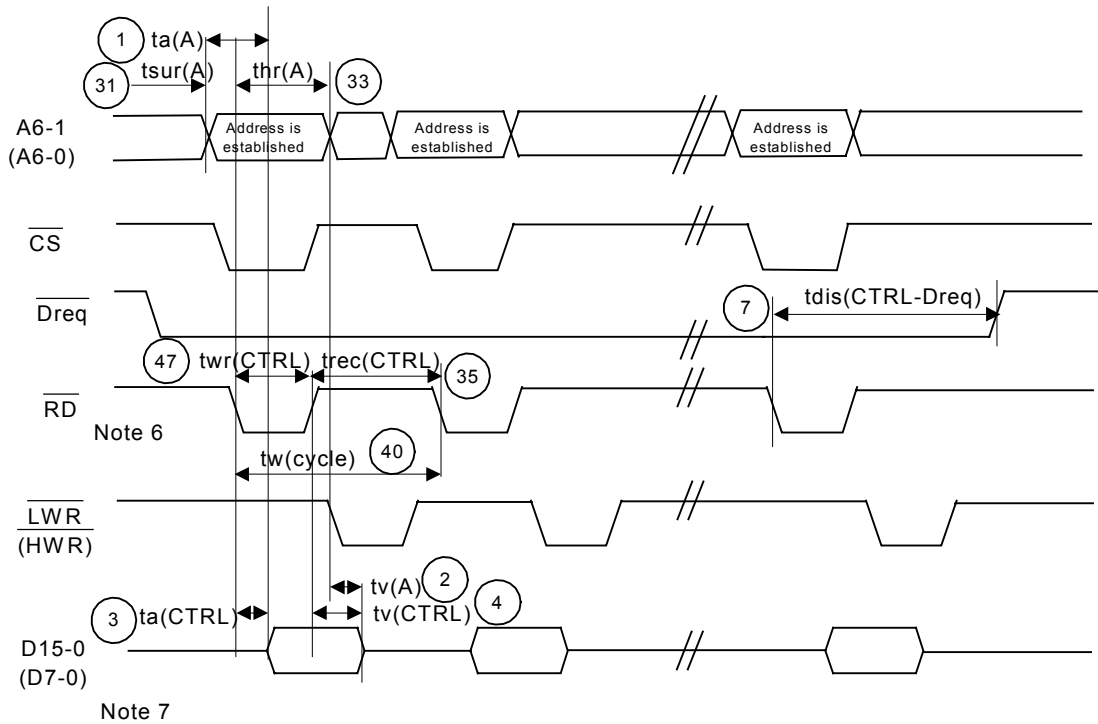
(3-4) Read timing (DMAEN=1, DFORM=10)
