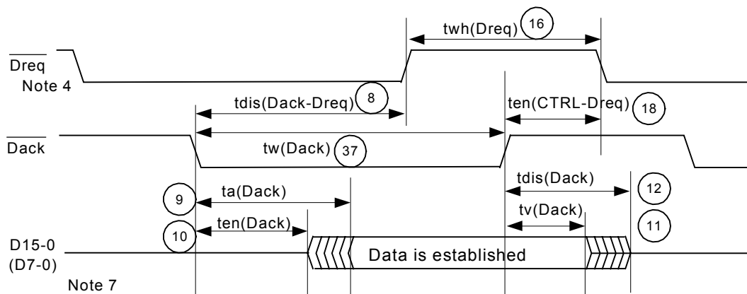
(2-4) Read timing 2 (DMAEN=1, DFORM=01)
