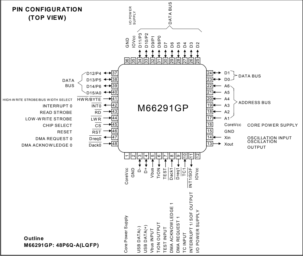
Figure 1.1 M66291 Pin Configuration
