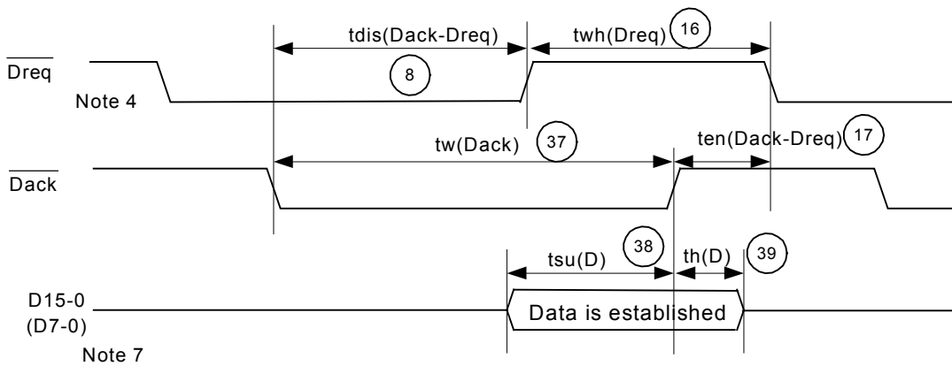
(2-3) Write timing 2 (DMAEN=1, DFORM=01)
