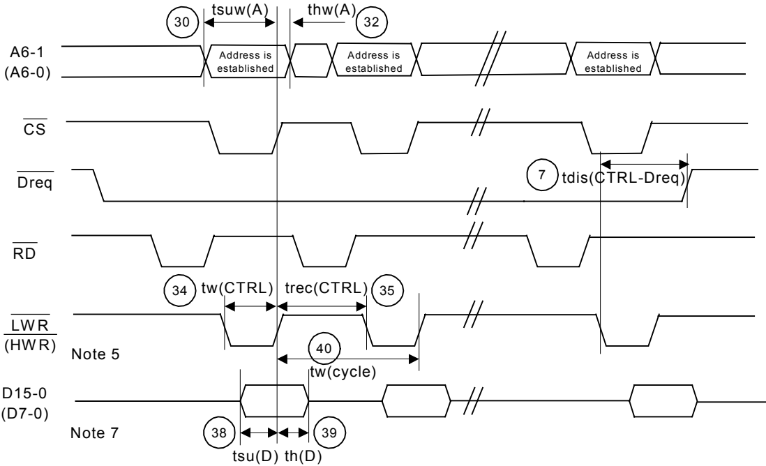
(3-3) Write timing (DMAEN=1, DFORM=10)
