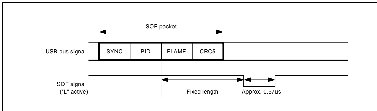
Figure 2.4 SOF Signal Output Timing
