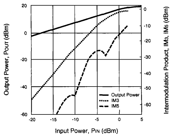
OUTPUT POWER AND INTERMODULATION PRODUCTS vs. INPUT POWER V_{DS} = 3 \text{ V}, I_{DS} = 20 \text{ mA}, f = 2 \text{ GHz}
