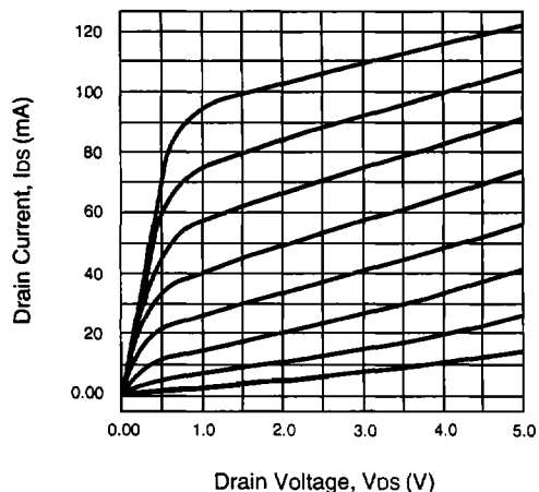
DC PERFORMANCE
