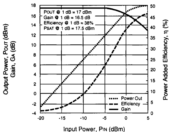
OUTPUT POWER, GAIN AND POWER ADDED EFFICIENCY vs. INPUT POWER V_{DS} = 3 \text{ V}, I_{DS} = 20 \text{ mA}, f = 2 \text{ GHz}
