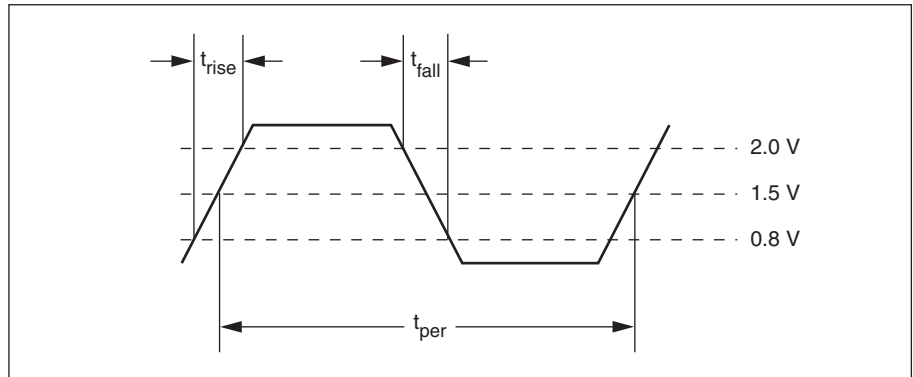
Figure 5-1. Input Waveform
