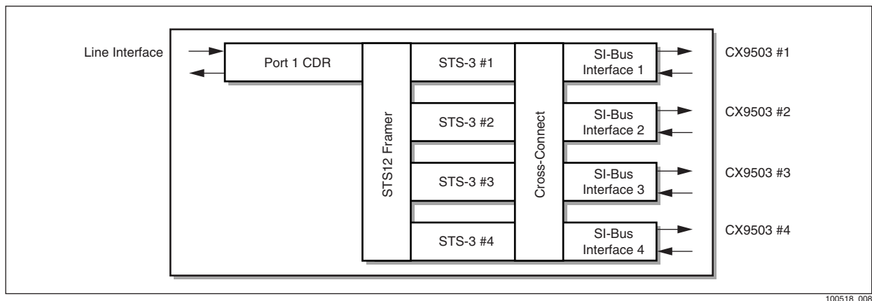
Figure 1-4. STS-12 Mode Data Flow Diagram
