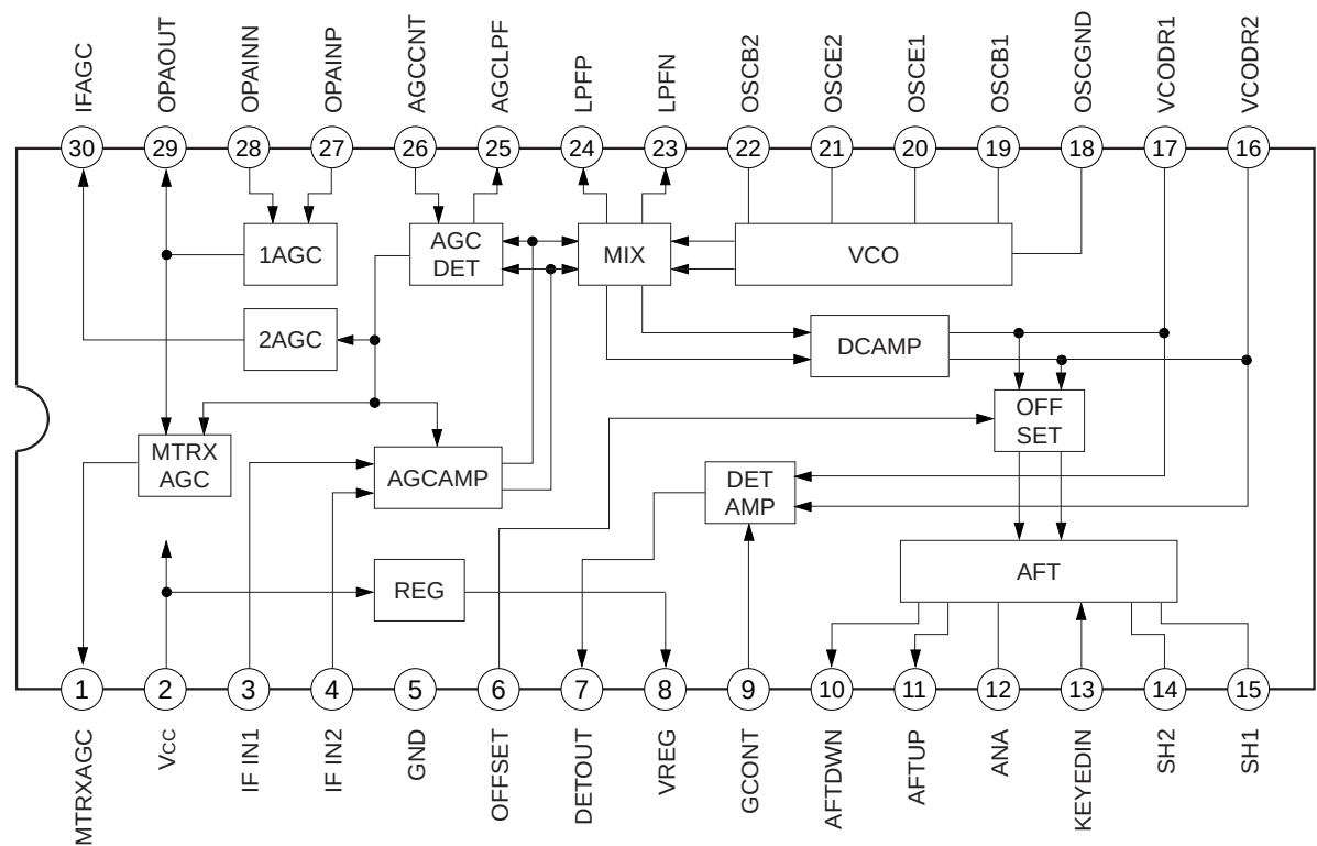
Block Diagram and Pin Configuration (Top View)
