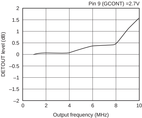
DETOUT characteristics
