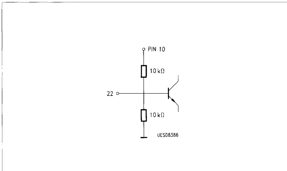
Figure 9 AF Operating Point PIN 22
