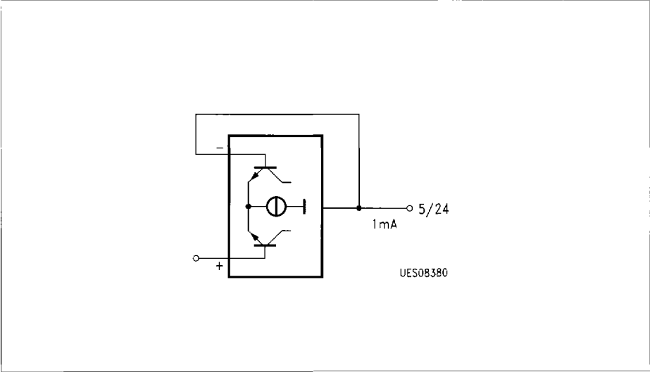
Figure 3 AF Outputs PIN 5/24
