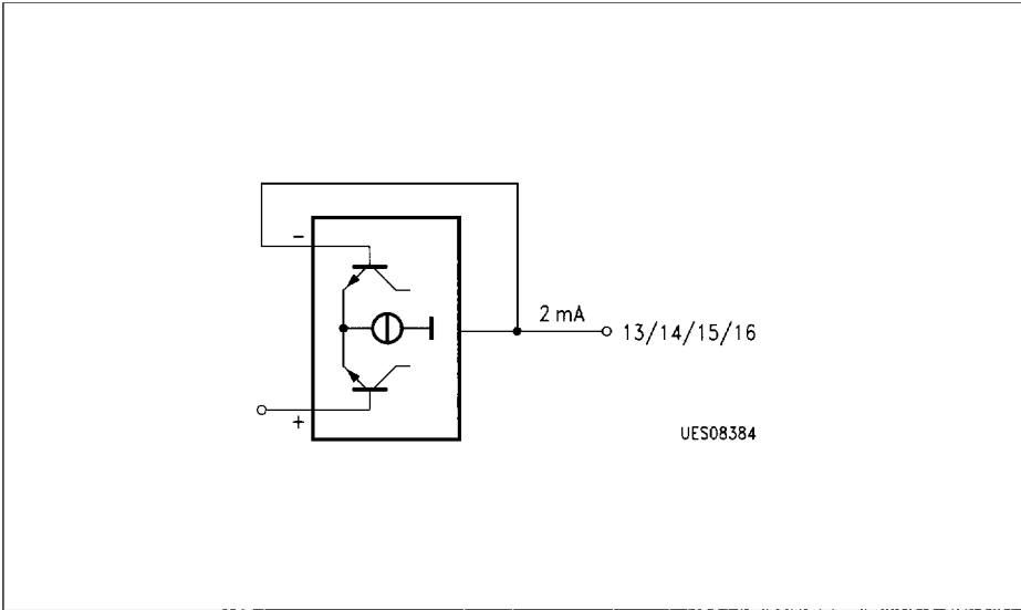
Figure 7 AF Outputs PIN 13/14/15/16
