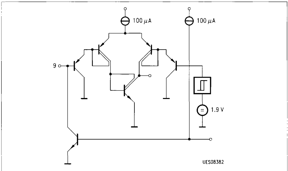
Figure 5 I 2 C Bus SDA PIN 9
