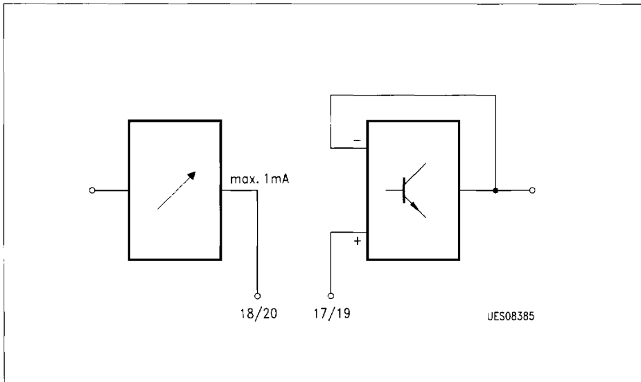
Figure 8 Corner Frequency Bass PIN 17/18/19/20
