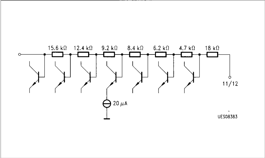
Figure 6 Corner Frequency Treble PIN 11/12
