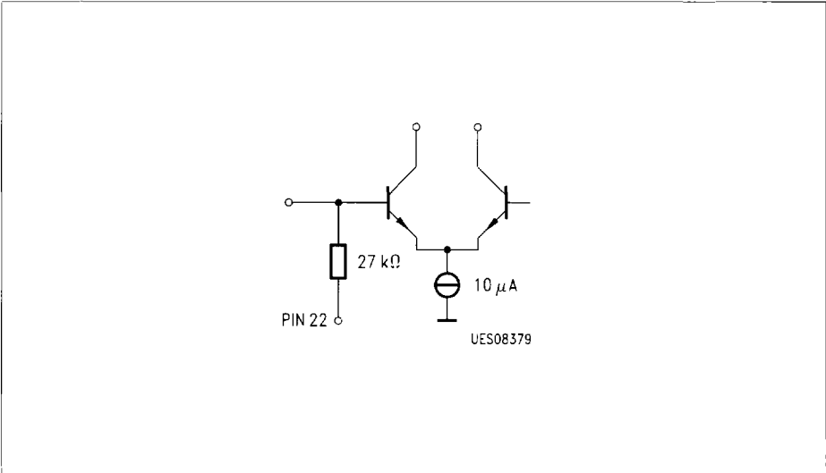
Figure 2 AF Inputs PIN 1/2/3/4/6/23/25/26/27/28
