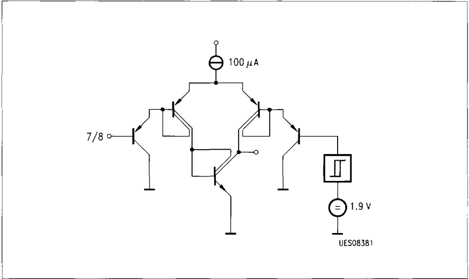
Figure 4 Reset PIN 7, I 2 C Bus SCL PIN 8
