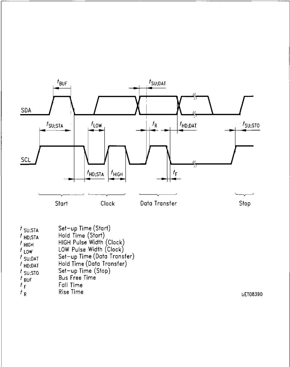
Figure 14 I 2 C Bus Timing
