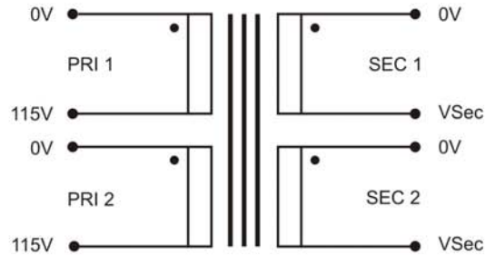
Schematic Diagram
