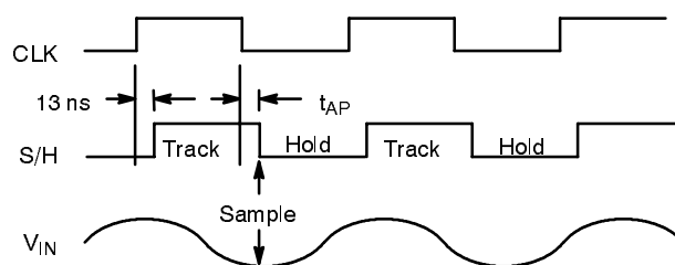
Figure 4. Sample and Hold Timing
