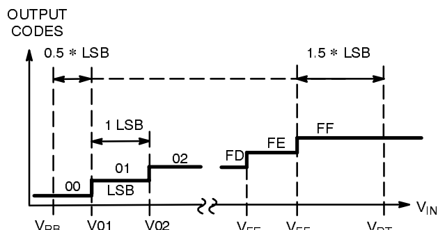
Figure 9. Ideal A/D Transfer Function
