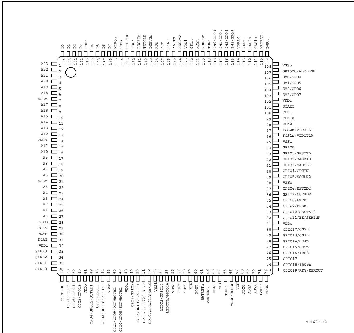
Figure 2. FC100/200 Pin Signals - 144-Pin TQFP
