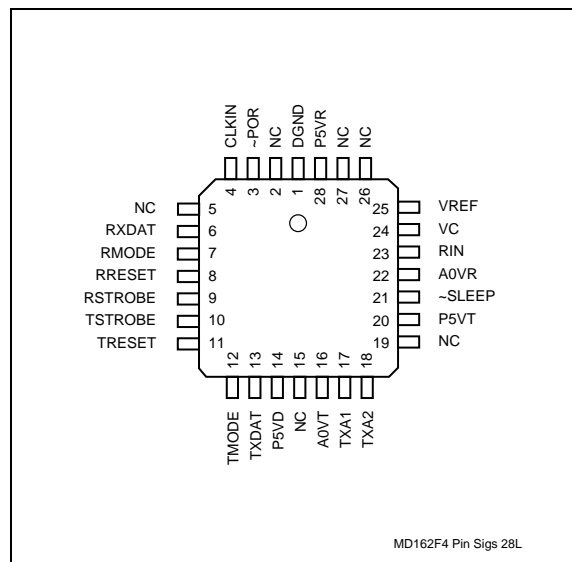
Figure 5. 28-Pin XIA Pin Signals
