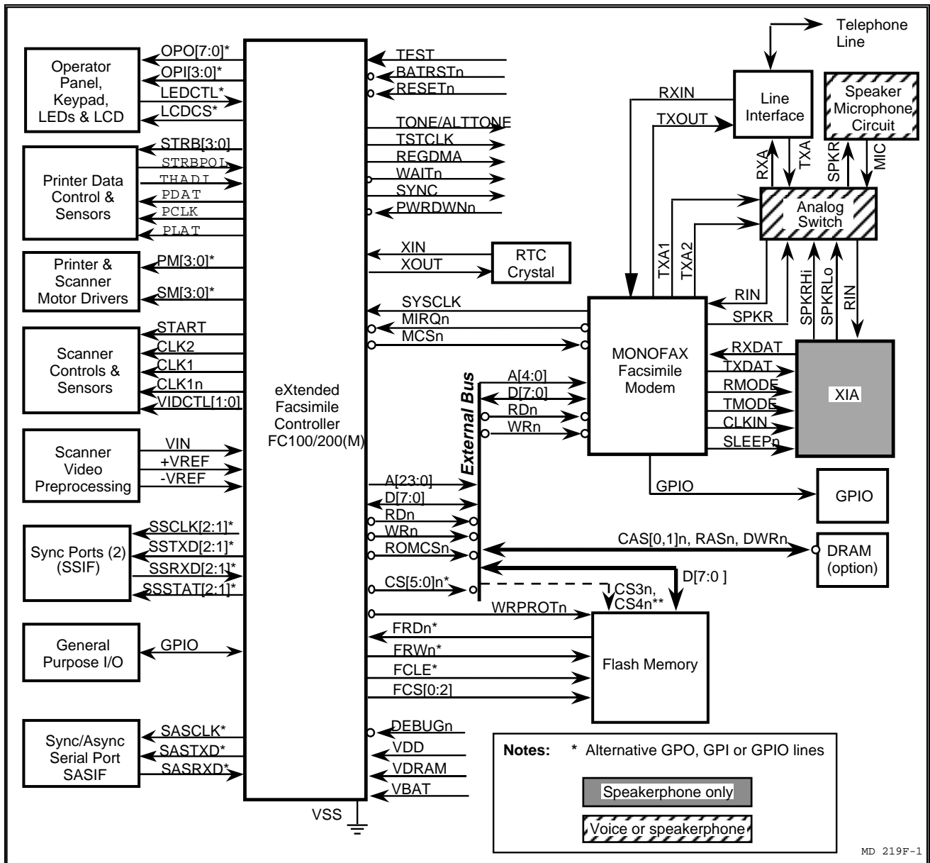
Figure 1. FE100/200 Functional Interconnect Diagram
